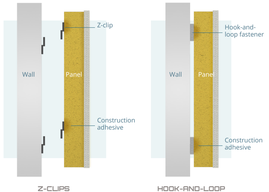
Z-CLIPS
