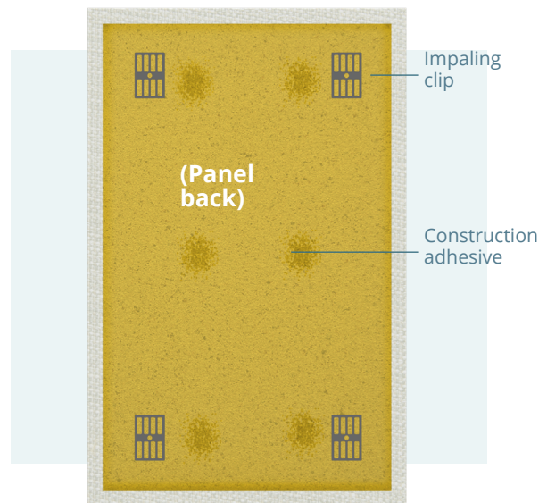
IMPALING CLIPS
